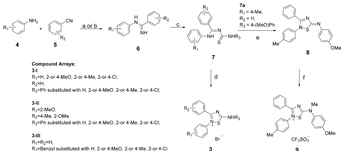
Scheme 1. (a) AlCl 3 /neat, 170–220 °C; (b) NaNH 2 , toluene, reflux; (c) R 3 NCS, 55 °C, 1,2-dichloroethane; (d) Br 2 , chloroform; (e) N -chlorosuccinimide, chloroform; (f) methyl triflate, dichloromethane.
