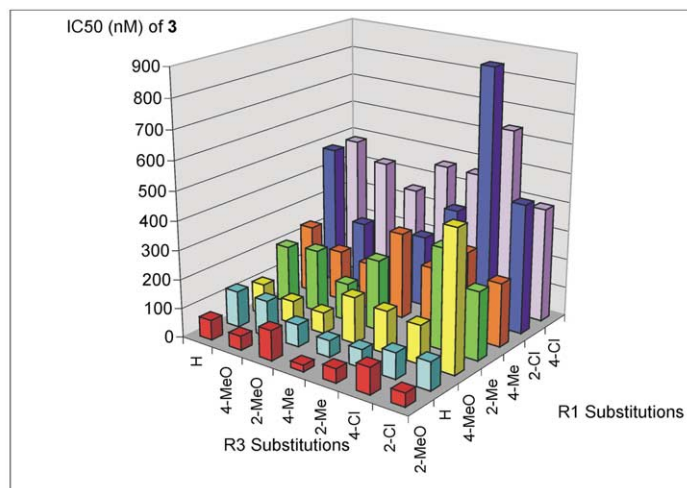
Figure 2. Binding affinities of 2-aryl-3-phenyl-5-anilino[1,2,4]thiadiazolium bromides 3 to the MC4 receptor—Part I.
