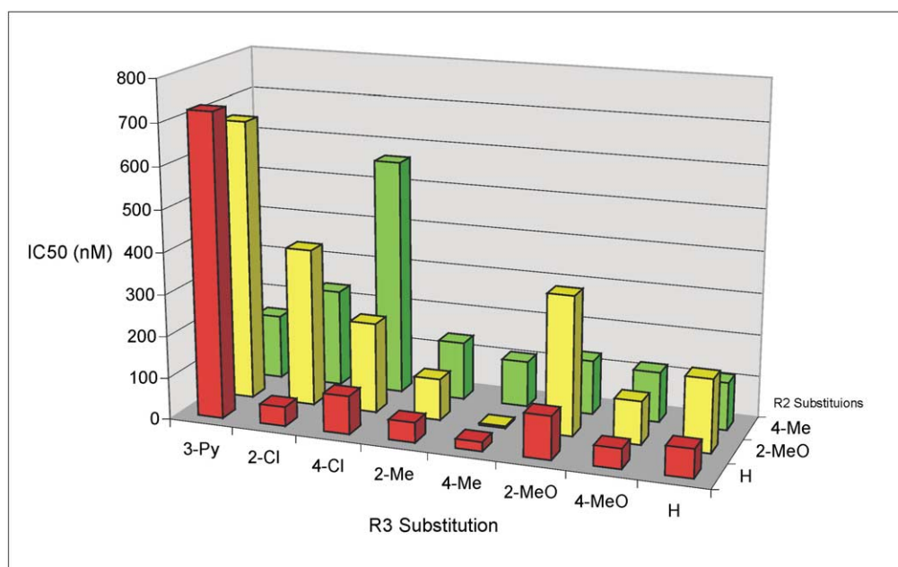
Figure 3. Binding affinities of 2-aryl-3-phenyl-5-anilino[1,2,4]thiadiazolium bromides 3 to the MC4 receptor—Part II.
